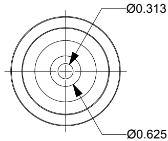
AFT END VIEW
